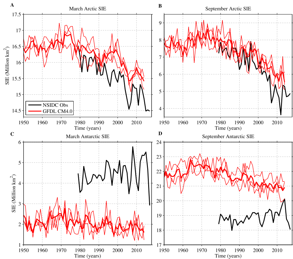
Figure 28. Time series of March and September Pan-Arctic (a,b) and Pan-Antarctic (c,d) sea ice extent (SIE; million km 2 ) from NSIDC satellite observations (black; Data Set ID: NSIDC-0051; Cavalieri et al., 1996), the three CM4.0 historical simulations (red), and the CM4.0 ensemble mean (thick red).
