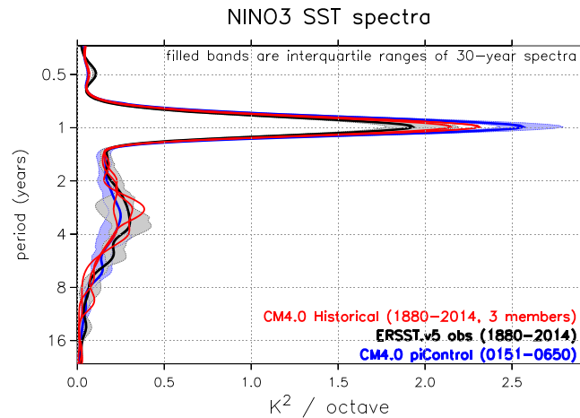
Figure 31. Power spectra of SST averaged over the Niño-3 region (150–90°W, 5°S–5°N), following Figure 2 of Wittenberg (2009). Abscissa indicates the time-averaged spectral power ( K^2 per octave) from a Morlet wave number 6 wavelet analysis. The area to the left of each curve represents the total spectral power within a given range of periods on the ordinate. Red lines are 1880–2014 time-mean spectra for the three CM4.0 historical ensemble members. Black curve is the 1880–2014 time-mean spectrum from the ERSST.v5 observational reanalysis (Huang et al., 2017); gray band indicates the interquartile range of ERSST.v5 sliding 30 year subspectra during 1880–2014. Blue curve is the CM4.0 preindustrial control run time-mean spectrum during Simulated Years 151–650; light blue band is the interquartile range of sliding 30 year spectra during that 500 year epoch.
